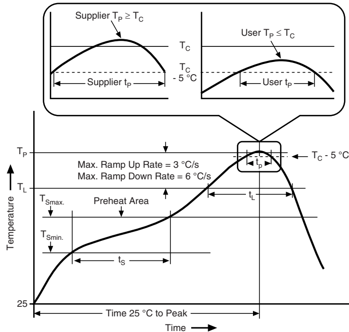
Reflow Soldering profile according to JEDEC® - J-STD-020D
