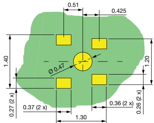
Footprint: CLP1515-5L (VSKY)
